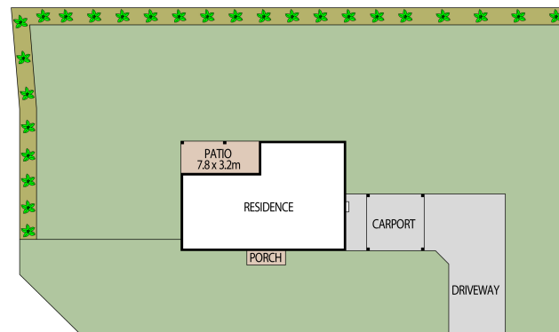
SITE PLAN
